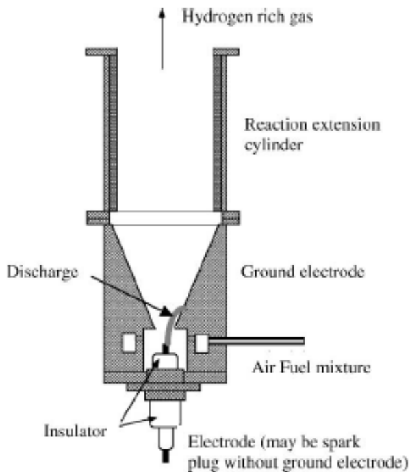
Figure 10: Low current plasmatron fuel reformer [14]
