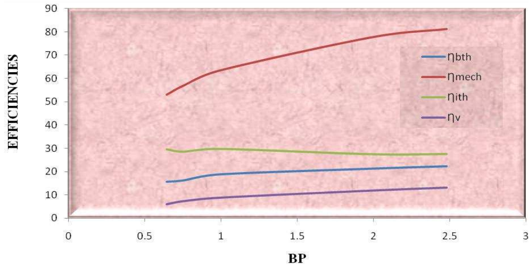
Graph 6. Variation of Brake Power (BP) with Efficiencies at 900 rpm
