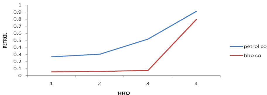
Graph 11. Variation of flow rate with carbon monoxide (CO) emissions for petrol and HHO gas
