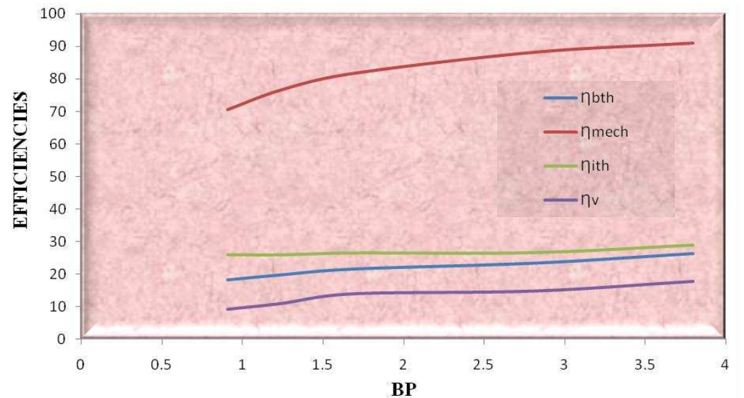
Graph 7. Variation of Brake Power (BP) with Efficiencies at 1100 rpm
