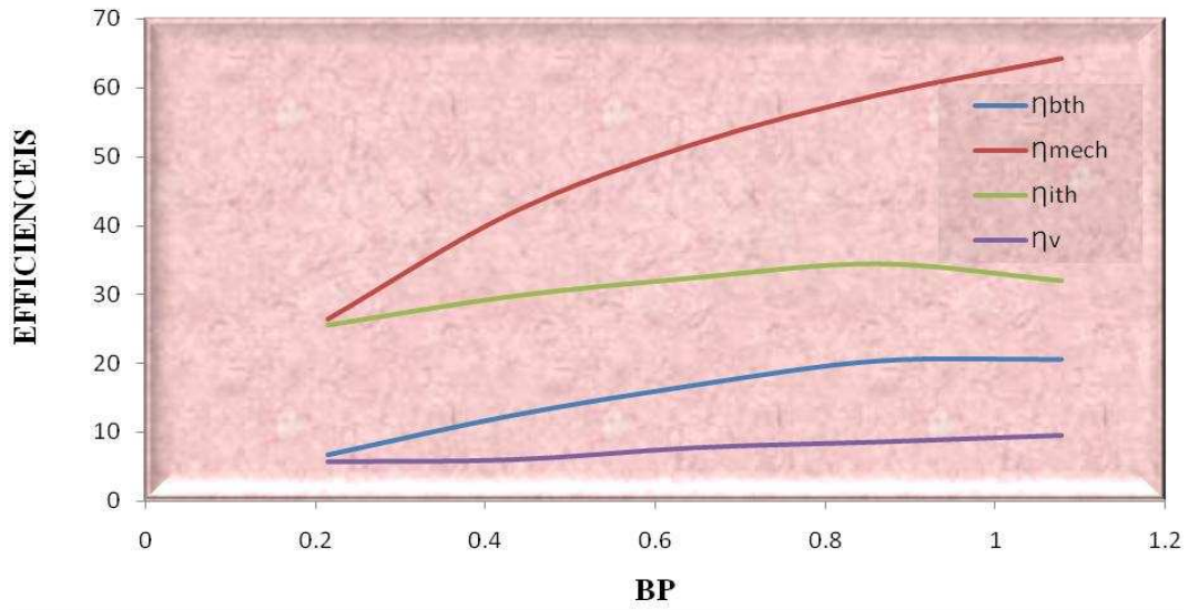
Graph 5. Variation of Brake Power (BP) with Efficiencies at 700 rpm
