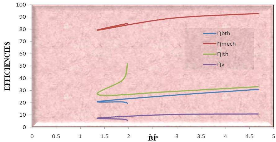
Graph 3. Variation of Brake Power (BP) with Efficiencies at 1100 rpm
