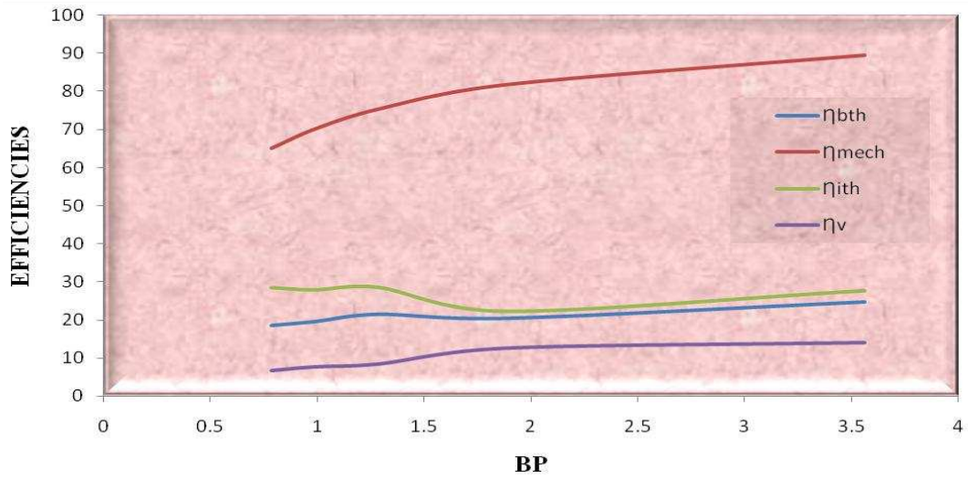
Graph 2. Variation of Brake Power (BP) with Efficiencies at 900 rpm
