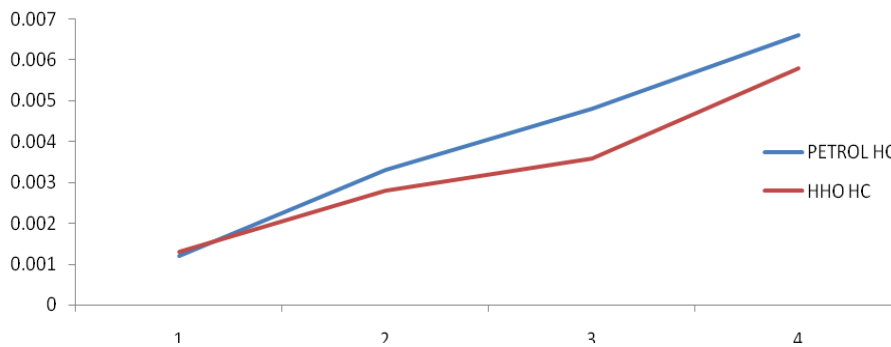
Graph 10. Variation of flow rate with hydrocarbon (HC) emissions for petrol and HHO gas
