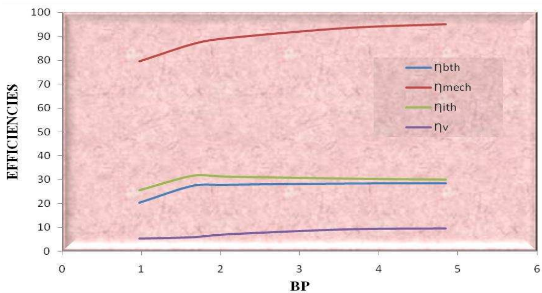
Graph 4. Variation of Brake Power (BP) with Efficiencies at 1300 rpm
