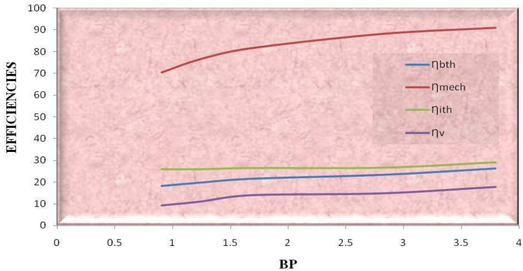
Graph 8. Variation of Brake Power (BP) with Efficiencies at 1300 rpm
