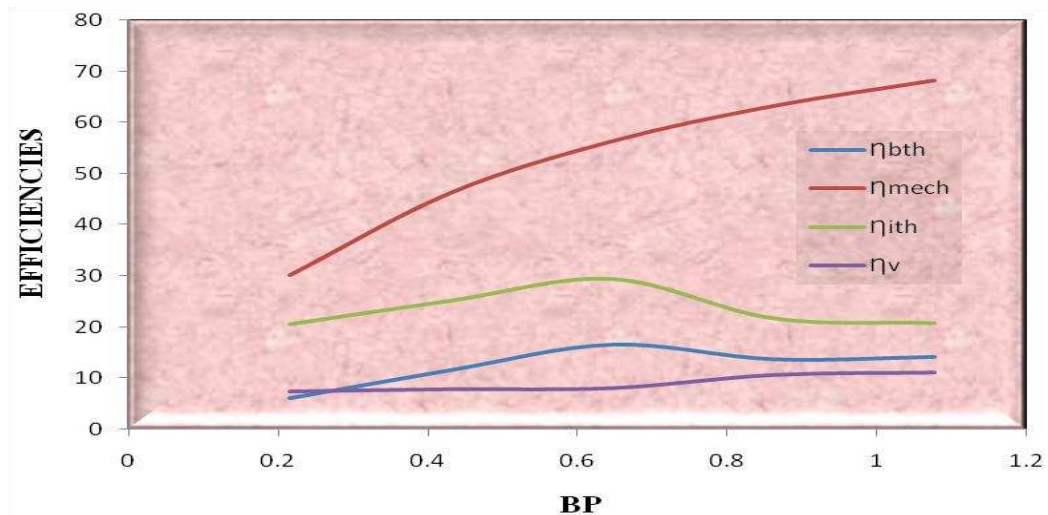
Graph 1. Variation of Brake Power (BP) with Efficiencies at 700 rpm
