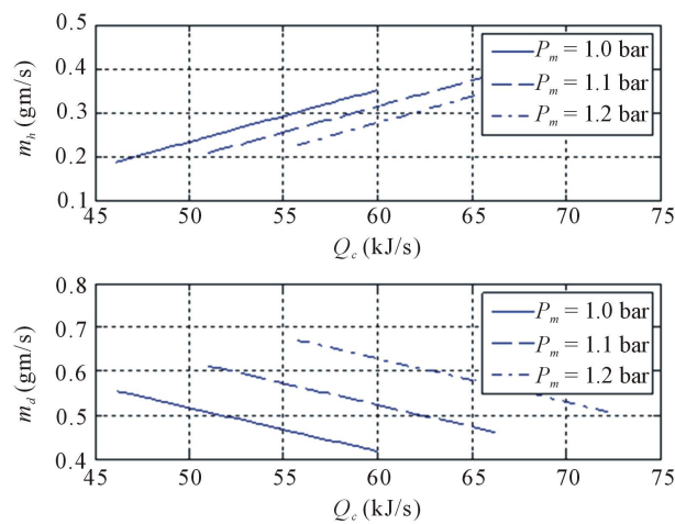
Figure 4. Variation of in-cylinder fuel energy with fuels mass flow with intake manifold pressure.
