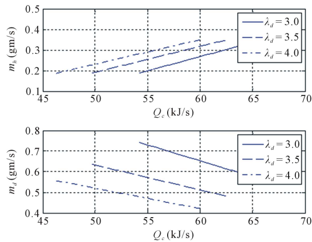
Figure 3. Variation of in-cylinder fuel energy with fuels mass flow and relative air-fuel ratio.
