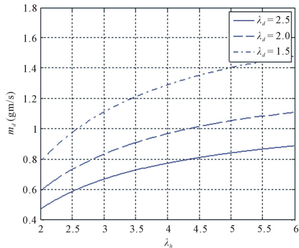
Figure 2. Variation of diesel mass flow with hydrogen and diesel relative air fuel ratio.
