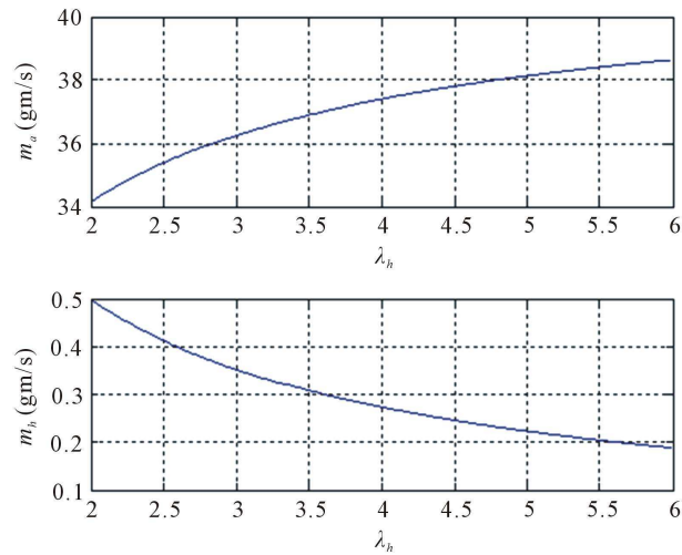
Figure 1. Variation of air and hydrogen mass flow with hydrogen relative air fuel ratio.
