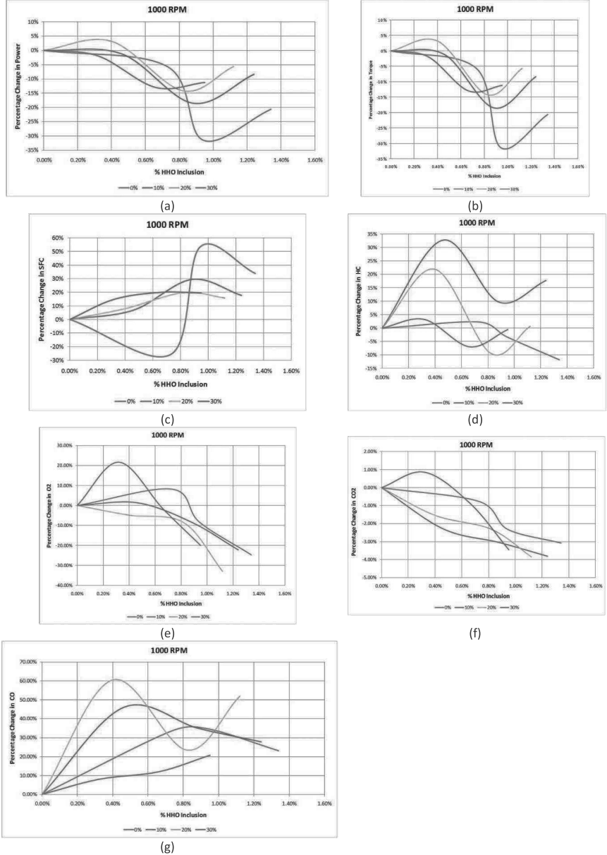
Figure 8: Response at 1000 rpm; (a) Power (b) Torque (c) SFC (d) HC (e) O 2 (f) CO 2 (g) CO
