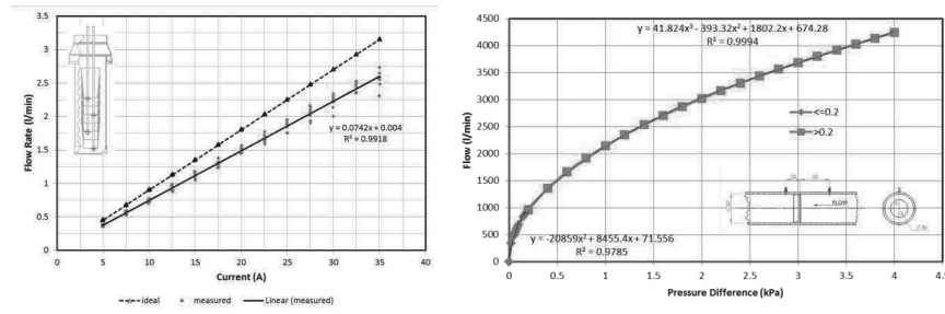
Figure 3: Calibration functions (a) HHO generator (b) Orifice plate
