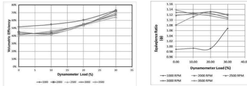
(a) (b) Figure 5: (a) Volumetric Efficiency (b) Equivalence ratio
