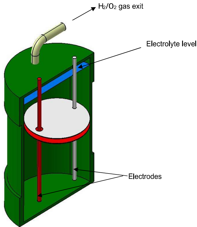
Figure 1: H 2 /O 2 generator section cut
